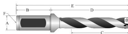
Helical Fluted Design
